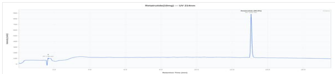
GLP-3 R 10mg - PL-RT10-14: UV Chromatogram
